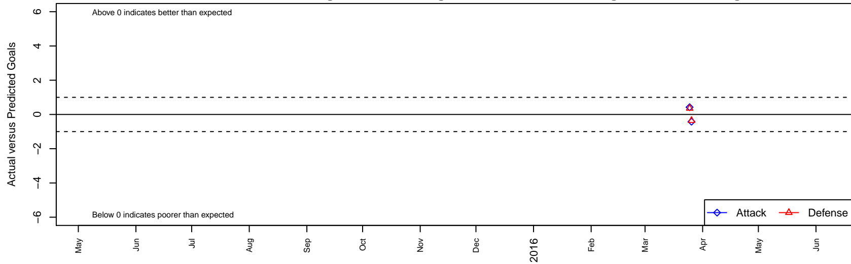
EMFC United 2001B Dots are actual minus expected GF (blue circles) and GA (red triangles). Blue line is smoothed change in attack strength. Red is smoothed change in defense strength.
